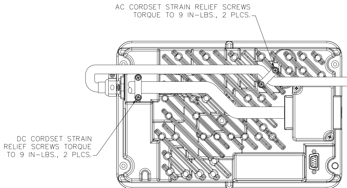
Figure 2-3: AC & DC Cordset Routing
